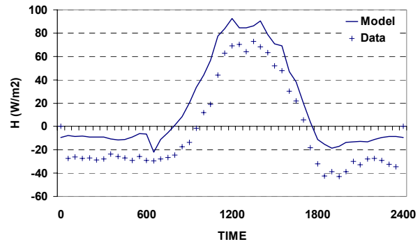
Diurnal cycle of sensible heat flux 199803
