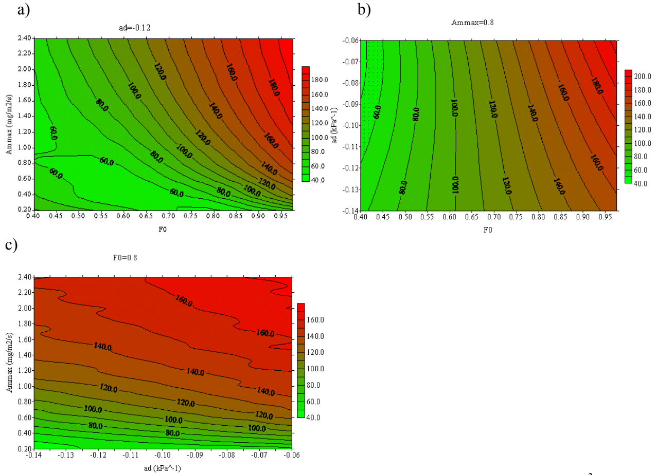
Figure 4.9: Contour plots of root mean square error (RMSE) for latent heat flux ( W/m^2 ) for Speuld96. a) A_{m,max}(@25) vs. f_0 with a_d = -0.12 kPa^{-1} , b) a_d vs. f_0 with A_{m,max}(@25) = 0.8 mg/m^2/s , c) A_{m,max}(@25) vs. a_d with f_0 = 0.80 .
