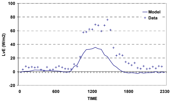
Diurnal cycle of latent heat flux 199811
