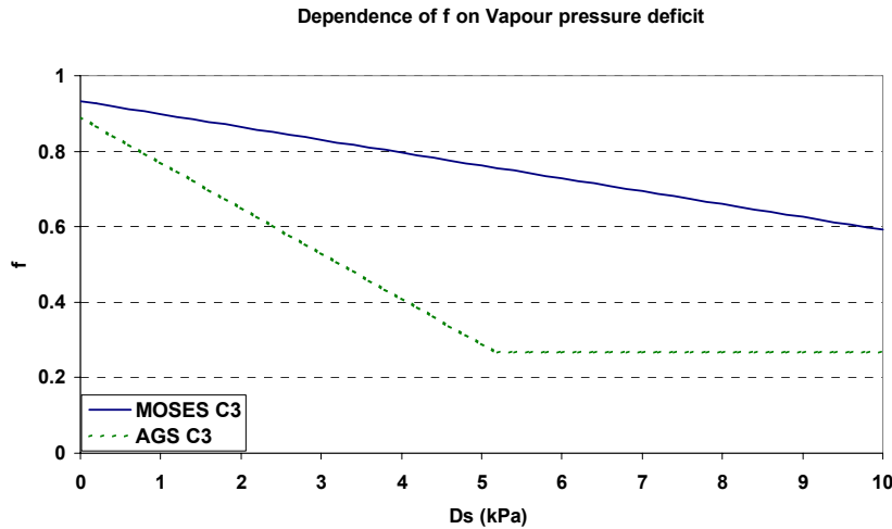
Figure 2.6: f as function of vapour pressure deficit for a C3 grassland modelled with MOSES and A-gs scheme with ceterus paribus values as in figure 2.5.
