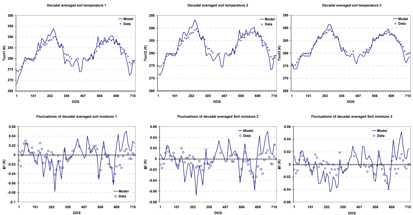
Figure 3.13: Time series for 1997 and 1998 of model results and data for soil variables in three layers: temperature and soil moisture (deviations from the mean value).
