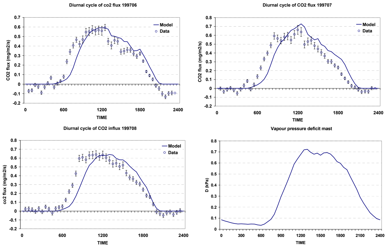
Figure 3.14: Diurnal cycles of modelled and measured CO 2 flux into the big-leaf during three summer months in 1997. The picture right below shows the diurnal cycle of measured vapour pressure deficit during July 1997.
