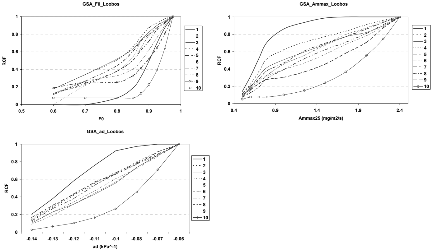
Figure 4.4: General sensitivity analysis for three parameters in the A-gs model, obtained from Loobos. The parameter is on the horizontal axis, the RCF on the vertical axis. Classes are shown with line appearances as indicated in the legend. Class 1 has the lowest RMSE and class 10 the largest RMSE
