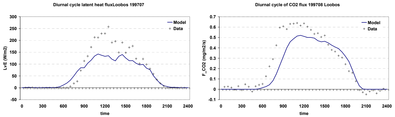
Figure 4.16: Diurnal cycle of fluxes of latent heat (left panel) and CO 2 (right panel) in Loobos.
