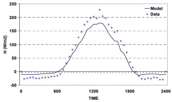
Diurnal cycle of sensible heat flux 199806
