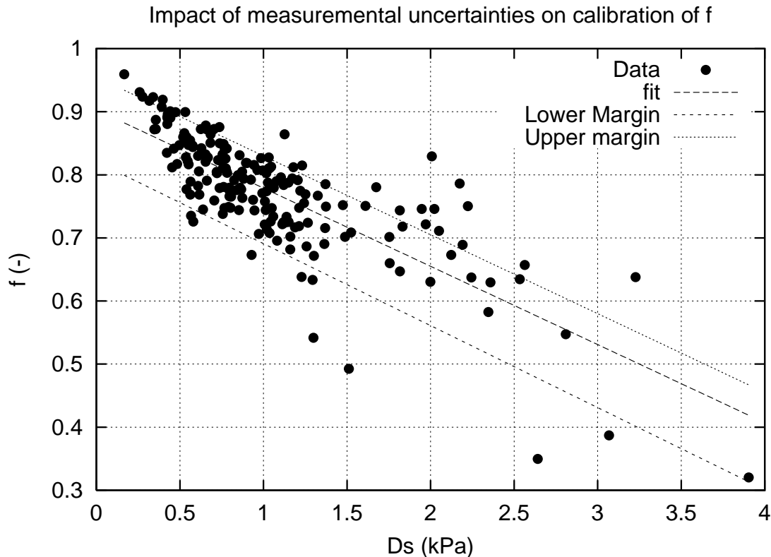
Figure 3.6. Effect of assuming measurement uncertainties on the calibration. Especially the intercept f_0 seems to be affected.
