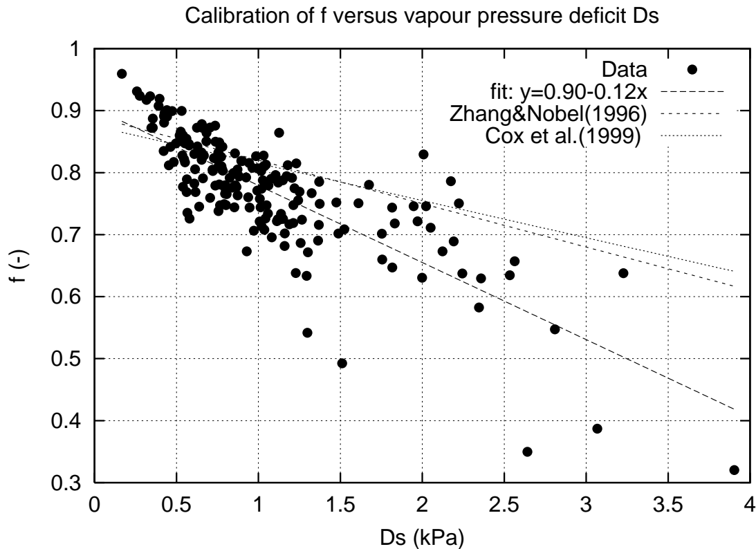
Figure 3.5: Results of the calibration of f versus the vapour pressure deficit. Also shown are functions by Zhang and Nobel (1996) and C99.
