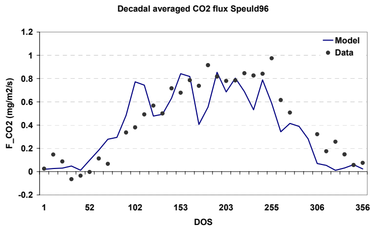
Figure 4.23: Time series of decadal averaged daytime CO 2 flux for Speuld96.
