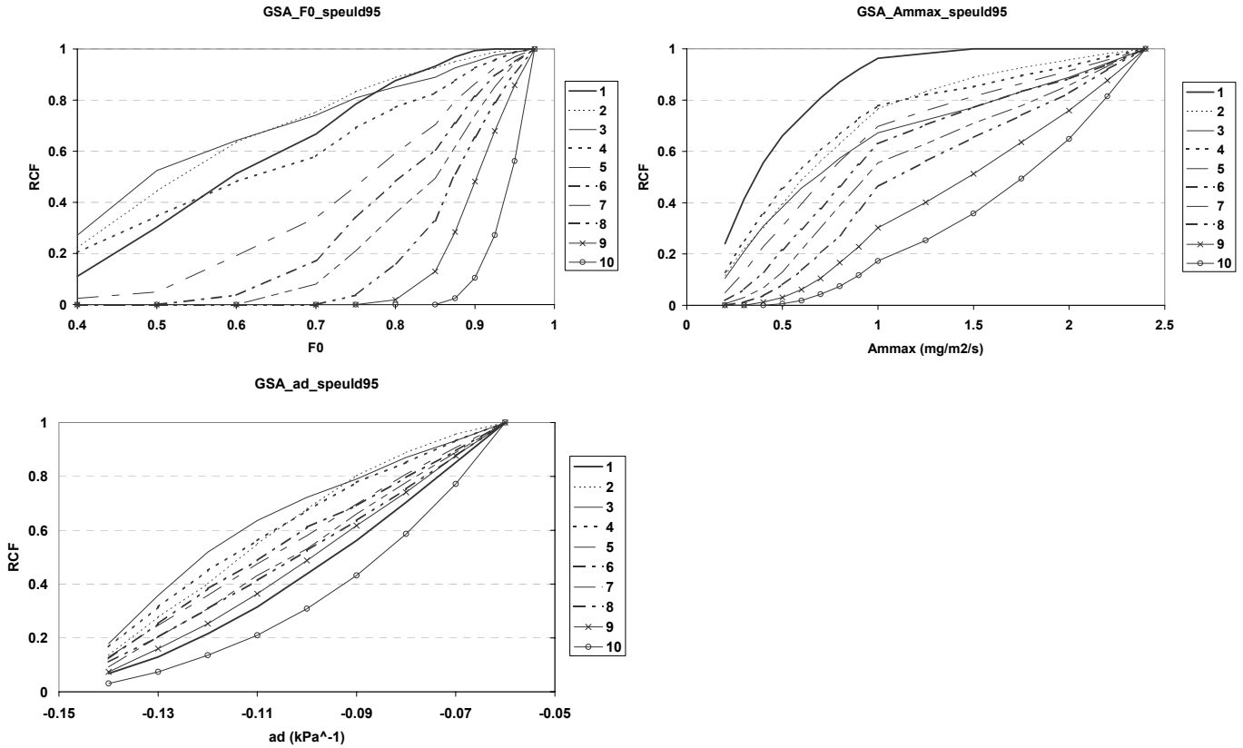
Figure 4.8: As in figure 4.4 for Speuld95.
