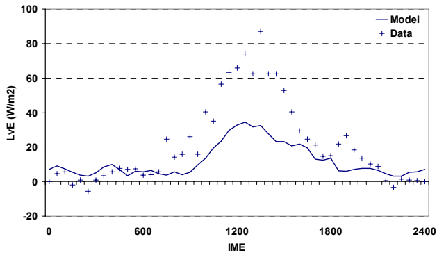
Diurnal cycle of latent heat flux 199801
