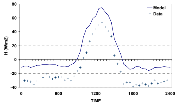
Diurnal cycle of sensible heat flux 199711
