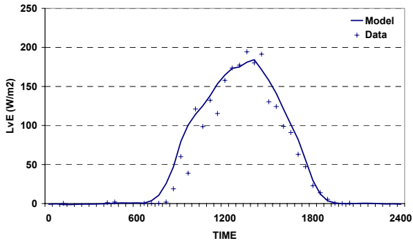
Diurnal cycle of latent heat flux 199709
