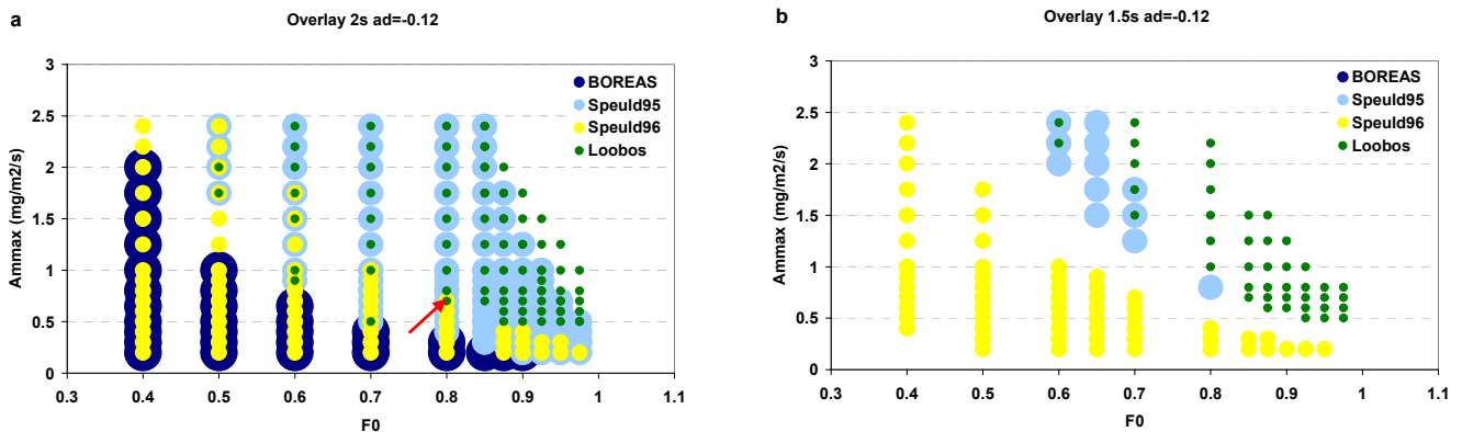
Figure 4.13: Overlay of the accepted parameter sets [f_0, A_{m,max}(@25)] for a_d = -0.12 \text{ kPa}^{-1} within a) 2\sigma_{LVE} and b) 1.5\sigma_{LVE} in the four forests.
