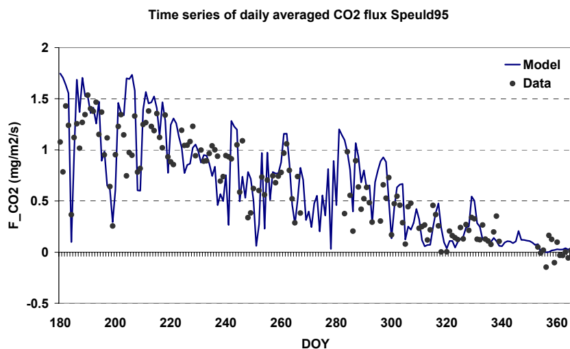
Figure 4.20: Time series of daily averaged daytime CO 2 flux for Speuld95.
