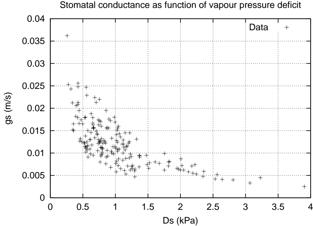
Figure 3.4: Dependence of stomatal conductance on vapour pressure deficit for Loobos
