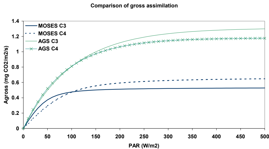
Figure 2.4: Comparison of gross assimilation in both models using parameter values as in literature.
