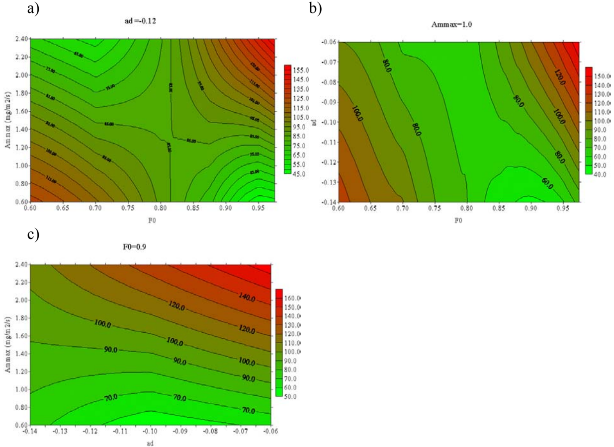
Figure 4.3: Contour plots of root mean square error (RMSE) for latent heat flux ( W/m^2 ) for Loobos. a) A_{m,max}(@25) vs. f_0 with a_d = -0.12 \text{ kPa}^{-1} , b) a_d vs. f_0 with A_{m,max}(@25) = 1.0 \text{ mg/m}^2/\text{s} , c) A_{m,max}(@25) vs. a_d with f_0 = 0.90 . These plots were made with the software package Surfer6.
