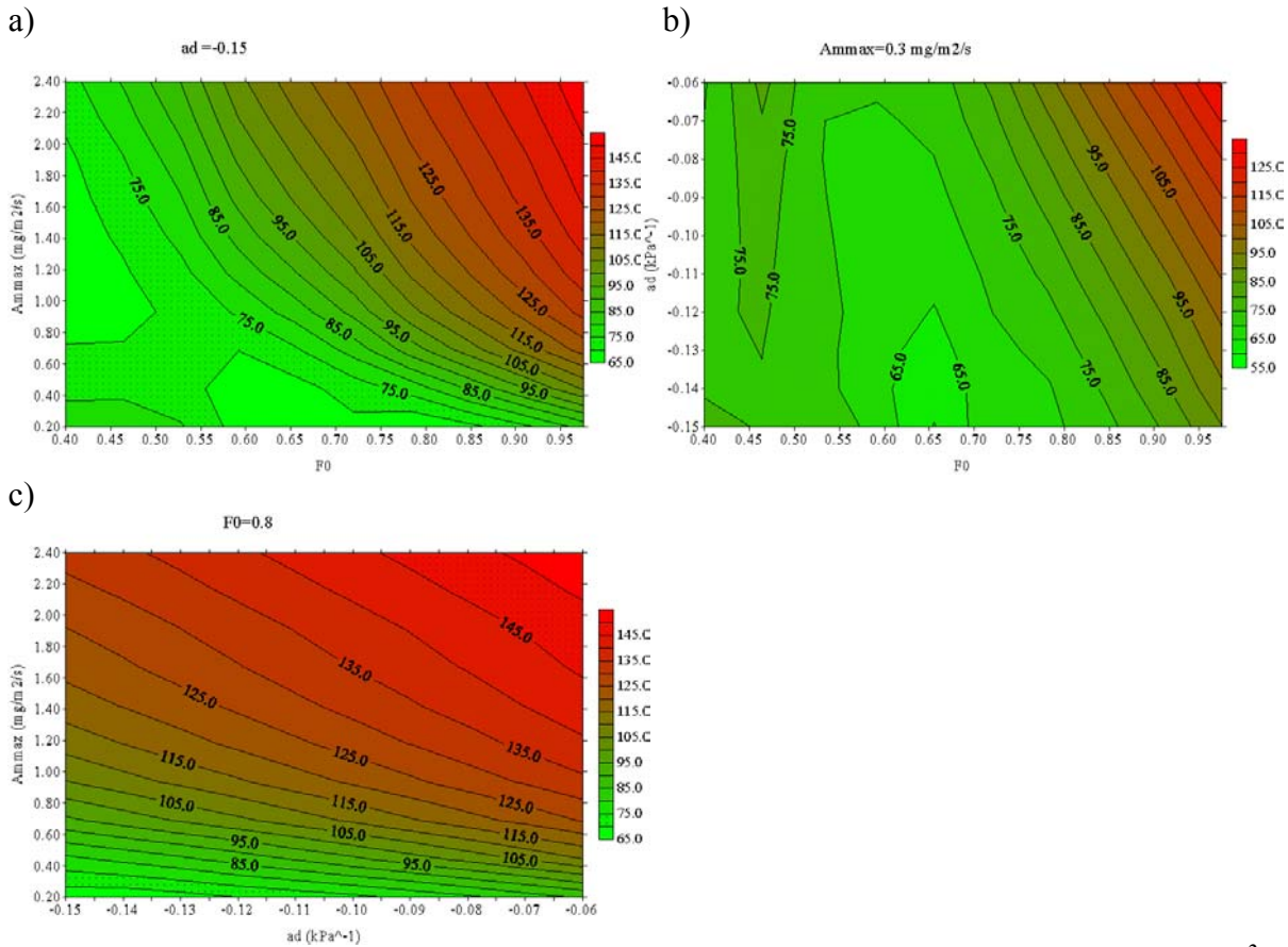
Figure 4.5: Contour plots of root mean square error (RMSE) for latent heat flux ( \text{W/m}^2 ) for BOREAS. a) A_{m,max}(@25) vs. f_0 with a_d = -0.15 \text{ kPa}^{-1} , b) a_d vs. f_0 with A_{m,max}(@25) = 0.3 \text{ mg/m}^2/\text{s} , c) A_{m,max}(@25) vs. a_d with f_0 = 0.80 .
