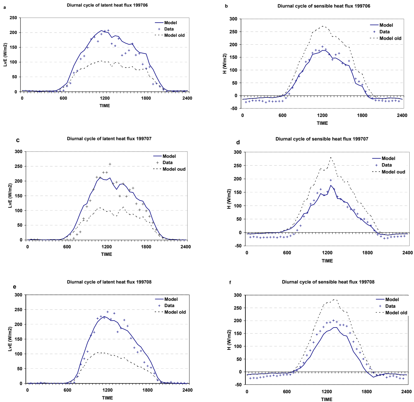
Figure 3.12: Comparison of diurnal cycle of latent and sensible heat flux with observations and the old A_g scheme for June 1997 (a & b), July 1997 (c & d) and August 1997(e & f).
