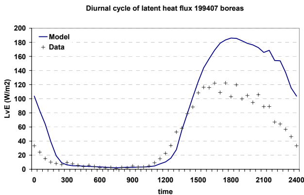
Figure 4.25: Diurnal cycle of latent heat flux for BOREAS.
