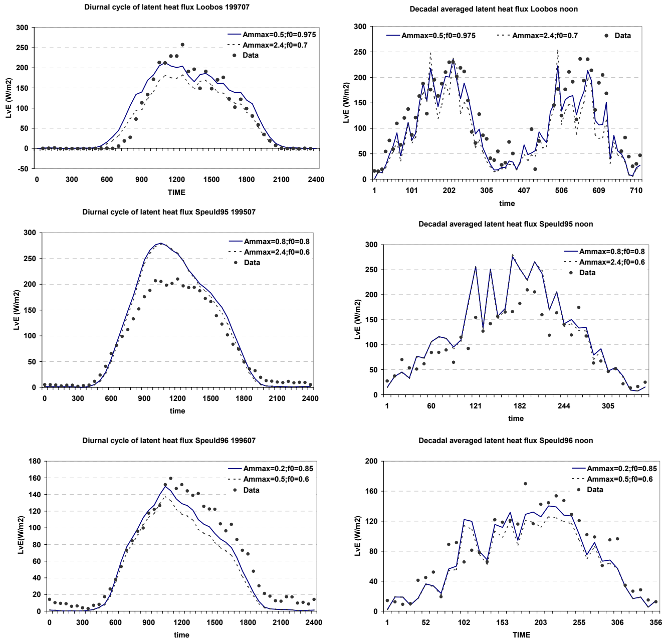
Figure 4.12 Time series (left panel diurnal cycle July, right panel decadal averages of time slots around noon) of latent heat flux for different parameter sets ( a_d = -0,12 \text{ kPa}^{-1} ) within the area of \sigma_{LVE} for Loobos, Speuld95 and Speuld96.
