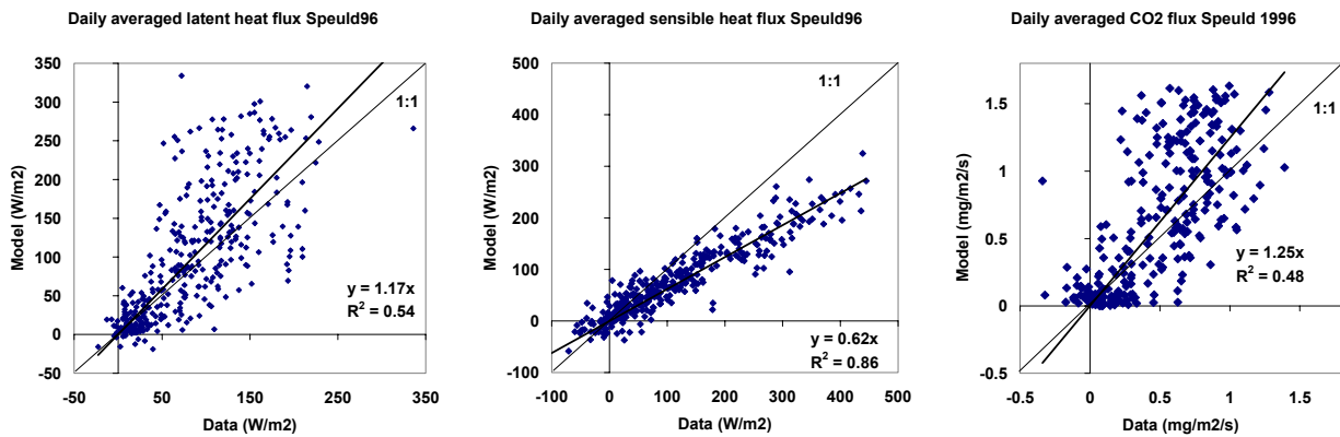
Figure 4.22: Daily averaged daytime fluxes of latent heat (left panel), sensible heat (middle panel) and CO 2 (right panel) for Speuld96.
