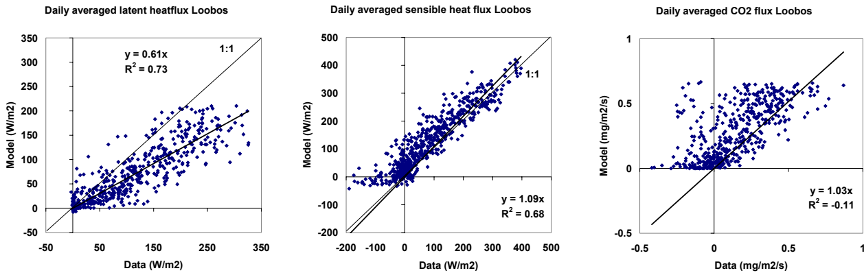
Figure 4.17: Daily averaged daytime fluxes of latent heat (left panel), sensible heat (middle panel) and CO 2 (right panel) for Loobos.
