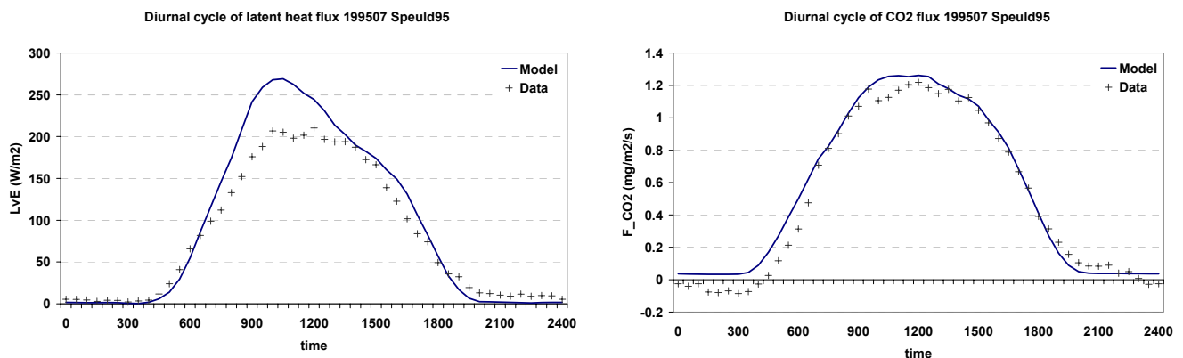
Figure 4.18: Diurnal cycle of fluxes of latent heat (left panel) and CO 2 (right panel) in Speuld95.
