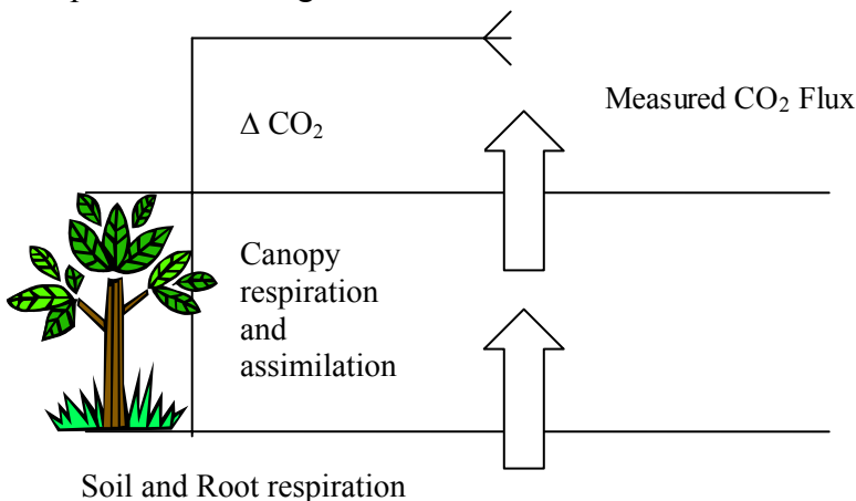
Figure 3.1: Illustration of CO 2 budgets.
