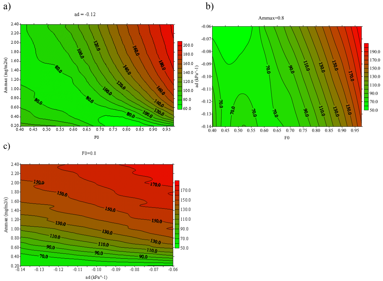
Figure 4.7: Contour plots of root mean square error (RMSE) for latent heat flux ( W/m^2 ) for Speuld95. a) A_{m,max}(@25) vs. f_0 with a_d = -0.12 kPa^{-1} , b) a_d vs. f_0 with A_{m,max} = 0.8 mg/m^2/s , c) A_{m,max}(@25) vs. a_d with f_0 = 0.80 .
