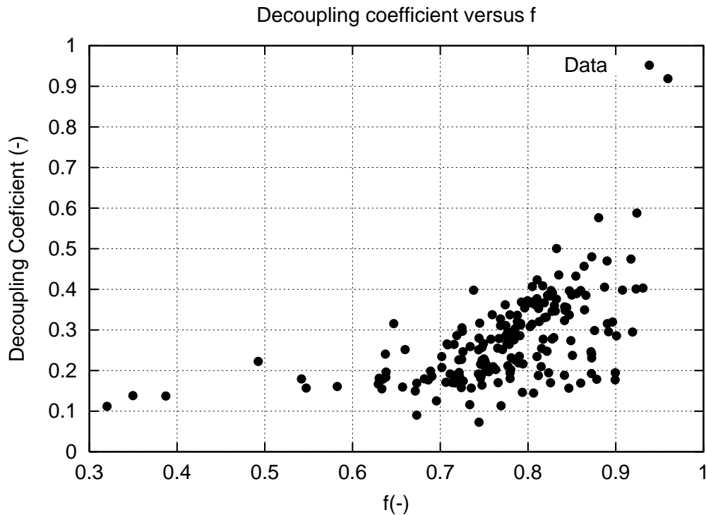
Figure 3.7: Decoupling between the forest and the atmosphere.
