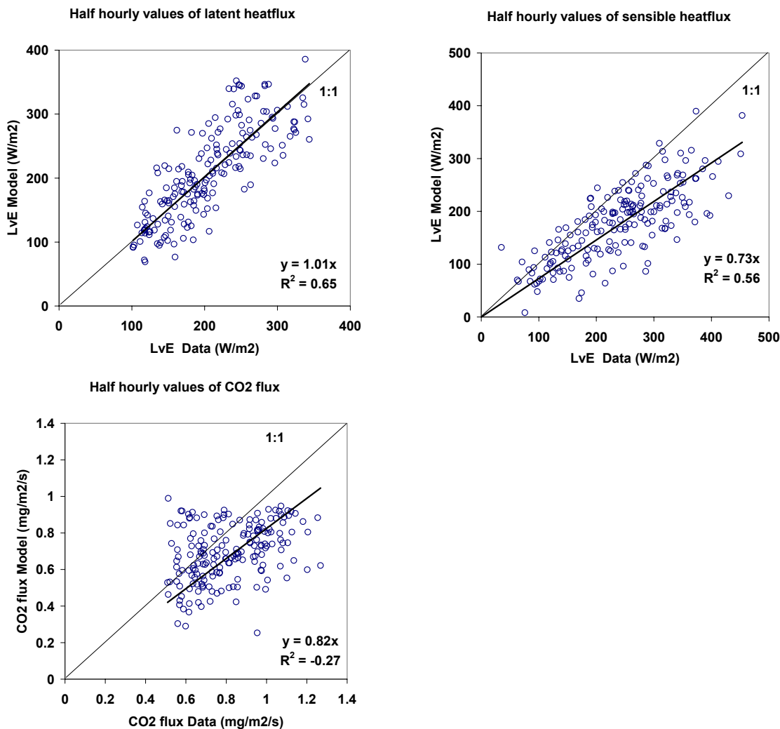
Figure 3.8: Scatter plots of latent- and sensible heat flux and CO 2 flux at leaf level for calibration points for the calibration of A_{m,max} and g_m .
