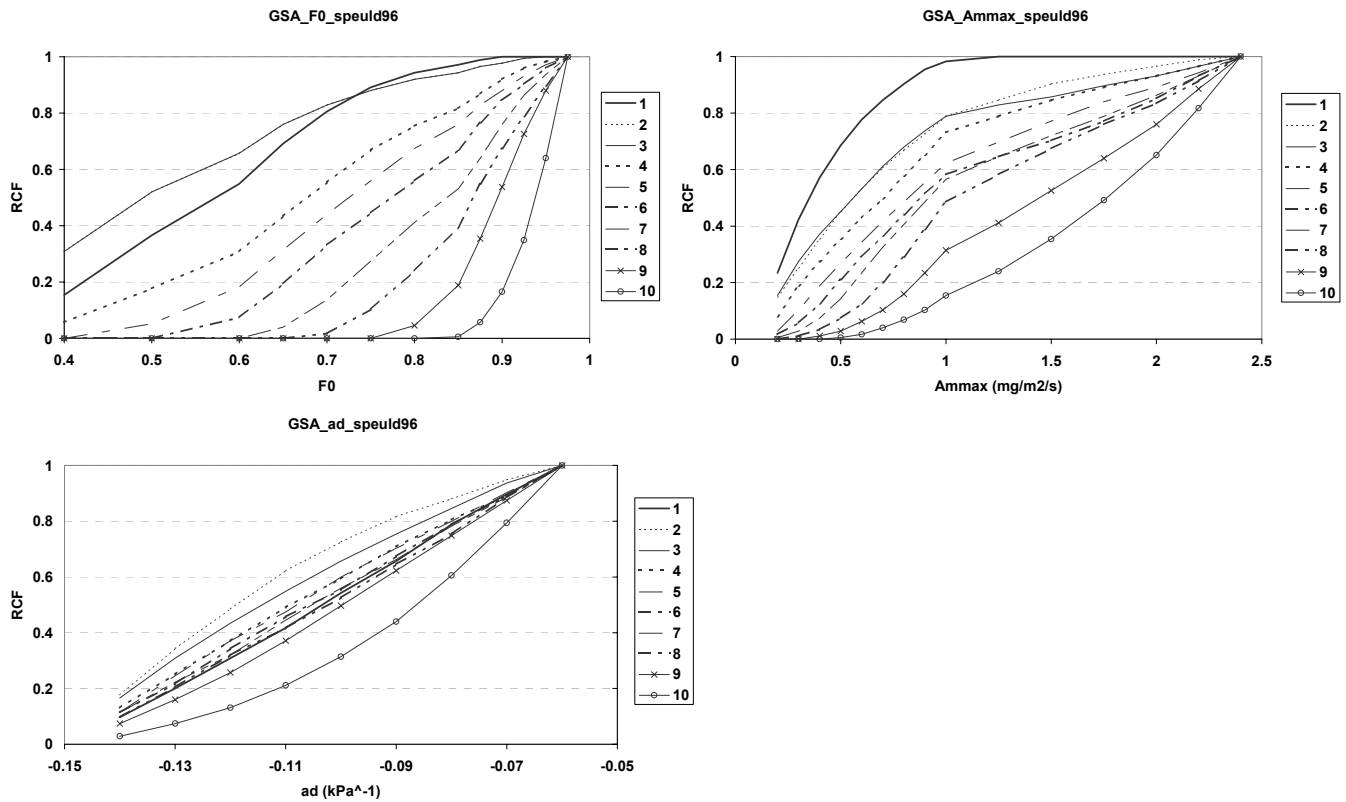
Figure 4.10: As in figure 4.4 for Speuld96.
