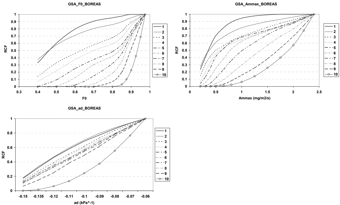
Figure 4.6: As in figure 4.4 for BOREAS.
