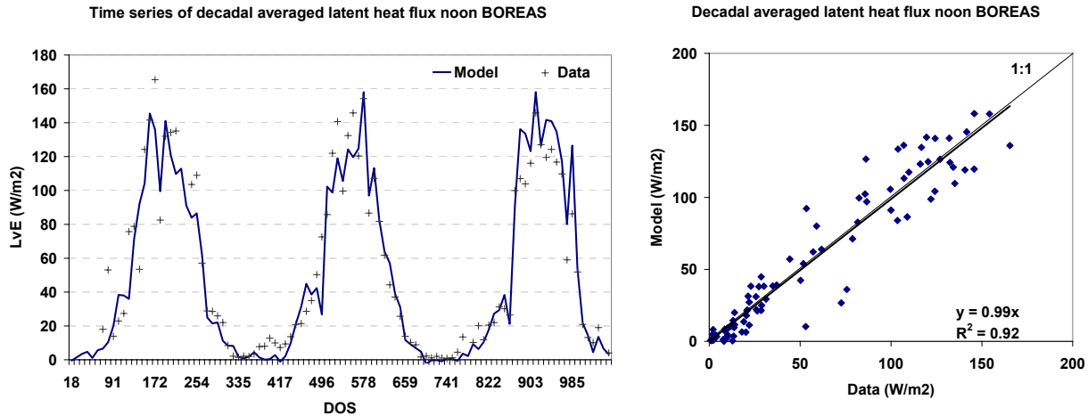
Figure 4.15: Time series of decadal averaged latent heat flux for BOREAS with parameter set: A_{m,max}(@25)=0.3 \text{ mg/m}^2/\text{s} , f_0=0.8 and a_d=-0.06 \text{ kPa}^{-1} .
