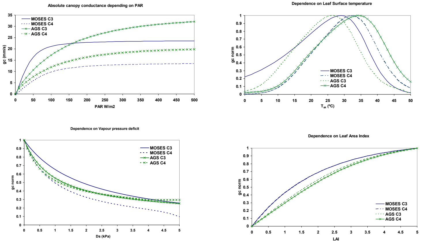
Figure 2.5: The sensitivity of canopy conductance to the environmental variables PAR, LAI, T_{sk} and D_s .
