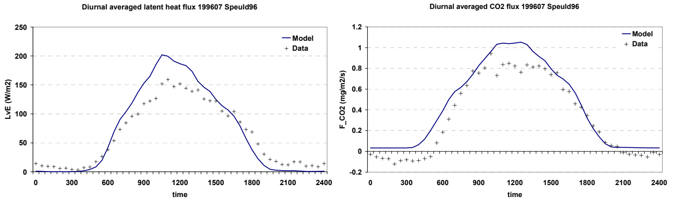
Figure 4.21: Diurnal cycle of fluxes of latent heat (left panel) and CO 2 (right panel) in Speuld96.
