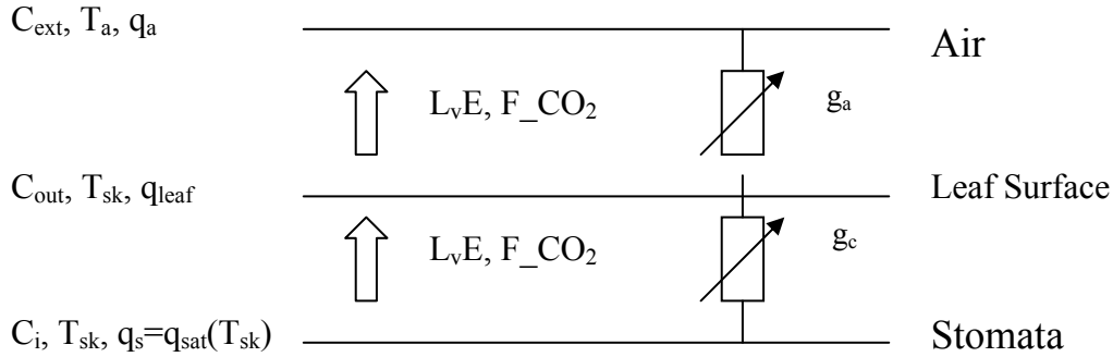
Figure 3.3: Resistance scheme for water vapour and CO 2 .
