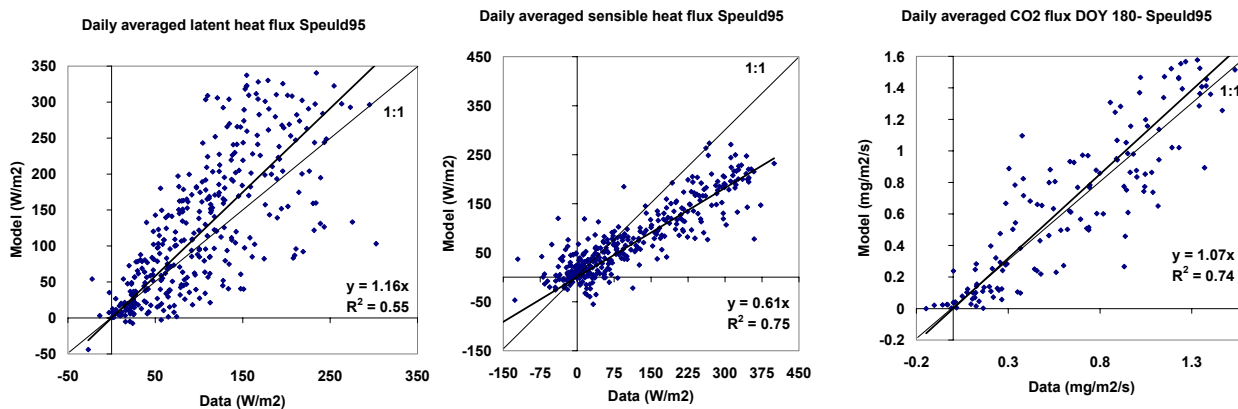
Figure 4.19: Daily averaged daytime fluxes of latent heat (left panel), sensible heat (middle panel) and CO 2 (right panel) for Speuld95.
