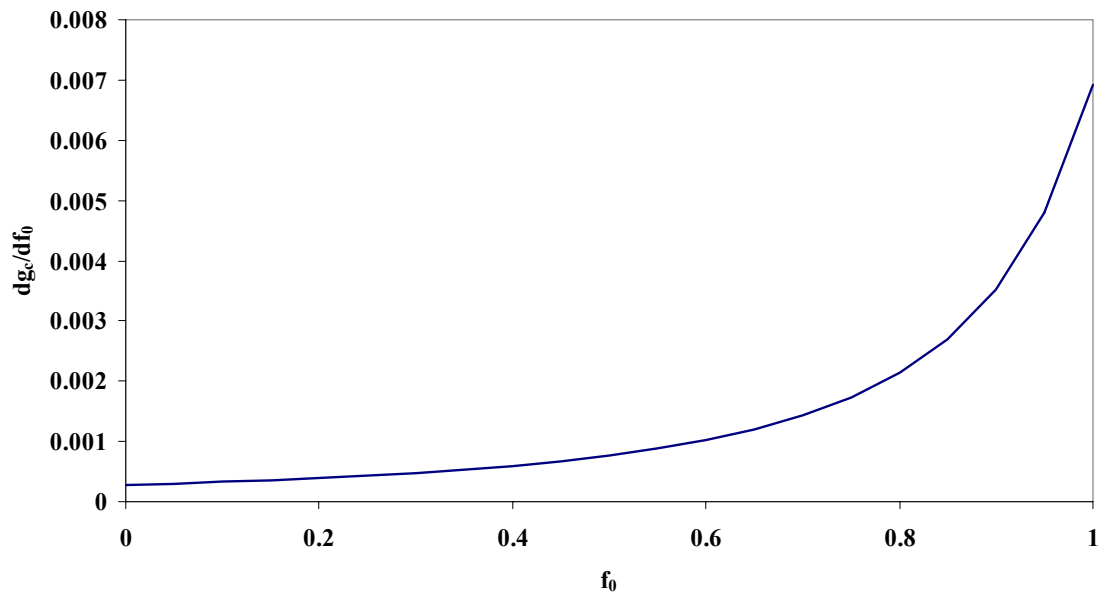
Figure E.1: The sensitivity of g_{b,c} for f_0 as function of f_0 . At large values of f_0 a larger sensitivity is obtained.
