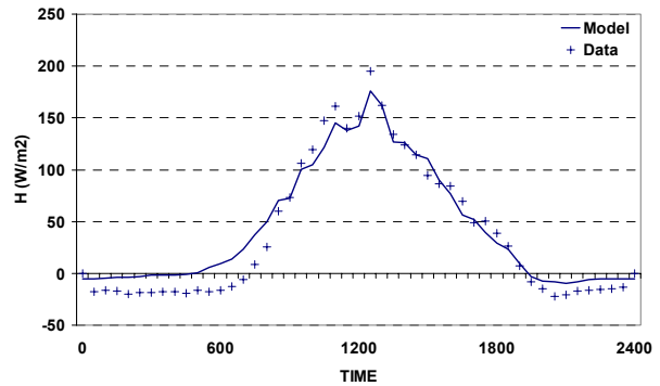
Diurnal cycle of sensible heat flux 199707
