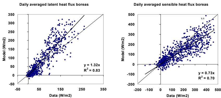
Figure 4.24: Daily averaged daytime fluxes of latent heat (left panel) and sensible heat (right panel) for BOREAS.
