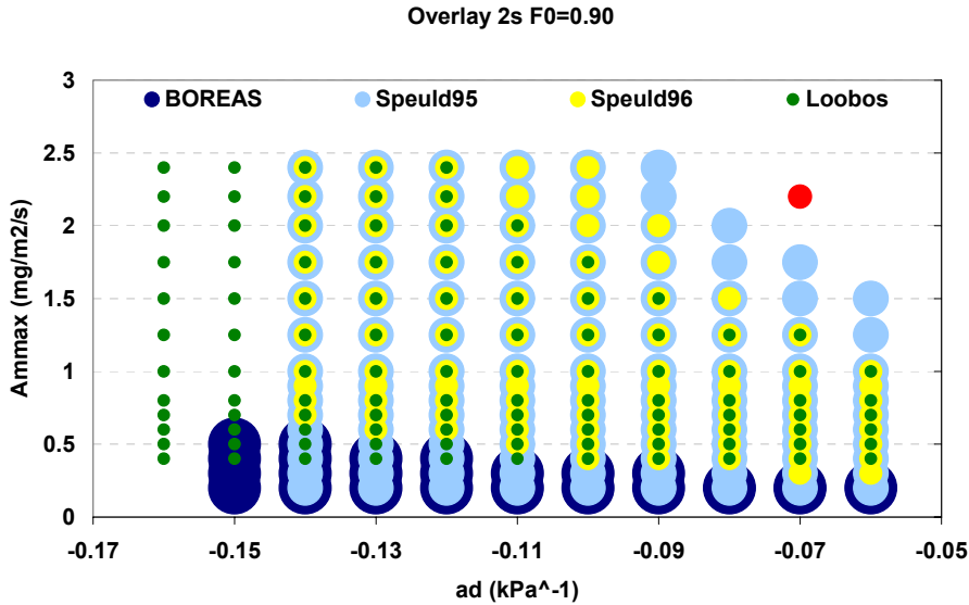
Figure 4.14: Overlay of the accepted parameter sets [A_{m,max}(@25), a_d] for f_0=0.90 within 2\sigma_{LVE} in the four forests. The red dot indicates the standard parameter values in the A-g scheme.
