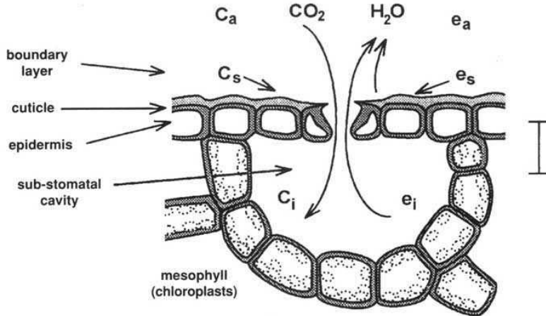
Figure 2.1: Cross section of a leaf stoma and \text{CO}_2 and water vapour fluxes. C stands for \text{CO}_2 concentration, e for water vapour pressure. Subscripts denote concentrations in free atmosphere ( a ), at leaf surface ( s ) and in the stomata ( i ).
