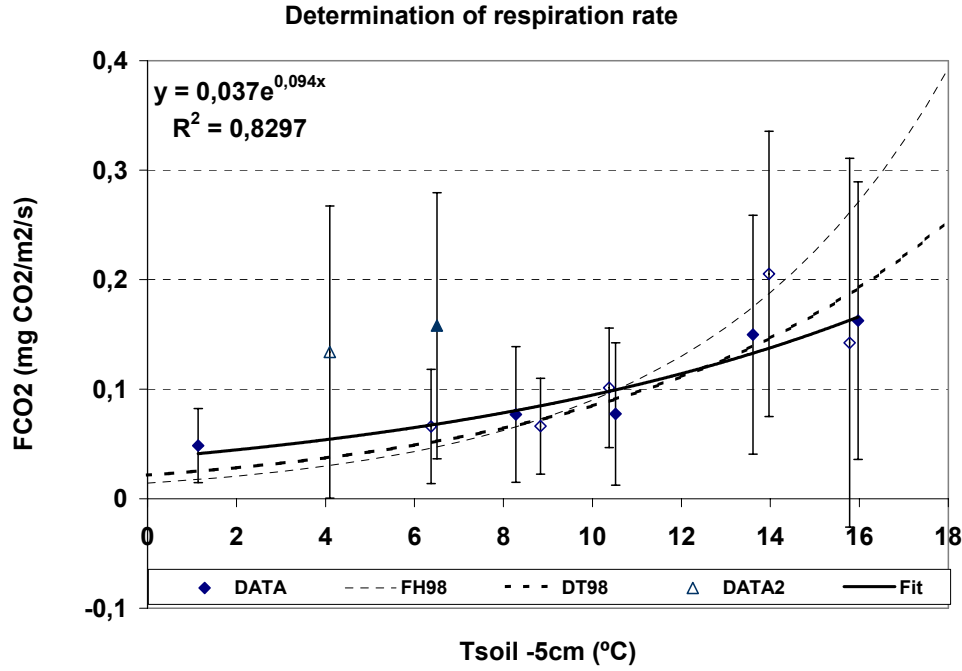
Figure 3.2: Determination of respiration processes as function of temperature. Open point indicators are 'wet' points, where solid indicators are the 'dry' points. An exponential curve is commonly used in literature. See e.g. Foster and Hadley (1998) and Davidson et al. (1998).
