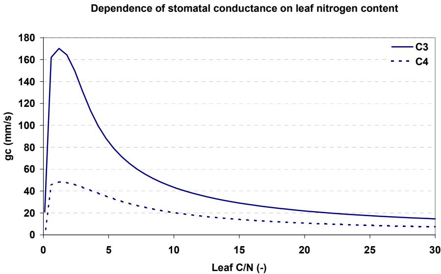
Figure 2.3: The influence of nitrogen content on canopy conductance in MOSES. PAR = 400 \text{ Wm}^{-2} , T_{sk} = 293 \text{ K} , LAI = 4 and D_s = 0 \text{ g/kg} .
