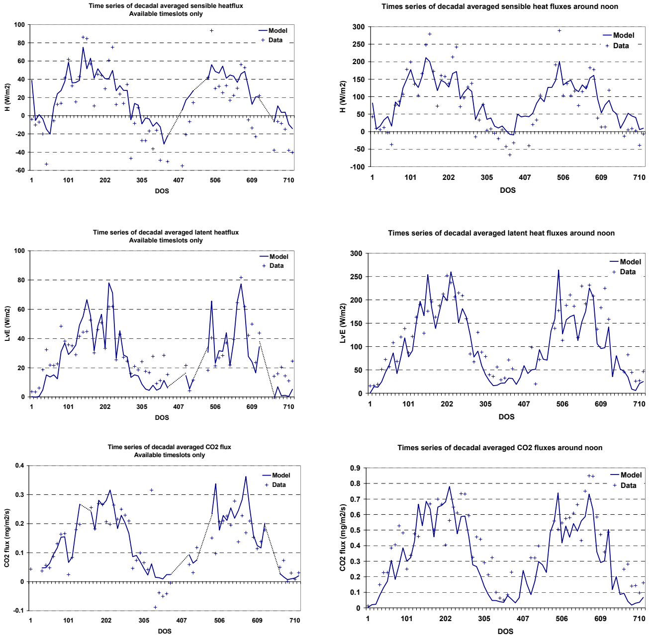
Figure 3.9: Time series of decadal averaged latent and sensible heat flux and CO 2 flux in 1997 and 1998. Left panels: averaged over whole day, right panels: averaged around noon: 10-14 local time.
