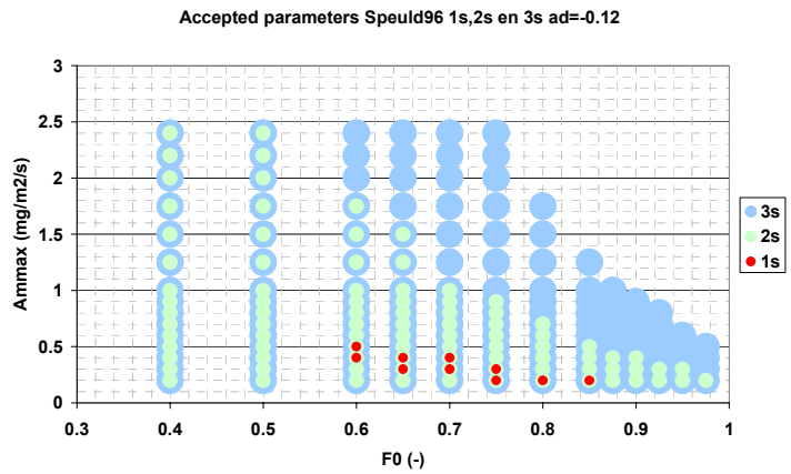
Figure 4.11: Accepted parameter values for Loobos, Speuld95, Speuld96 and BOREAS for varying significance levels. Red means that RMSE < \sigma_{LVE} ( 1.5\sigma_{LVE} for Speuld95), green that RMSE < 2\sigma_{LVE} and blue that RMSE < 3\sigma_{LVE} . Note that for BOREAS no red points are present.
