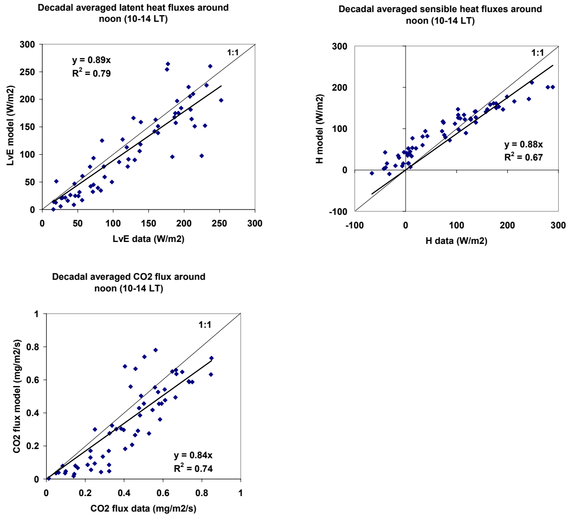
Figure 3.11: Idem as 3.10 but averaging took place only with data around noon (10-14 local time).
