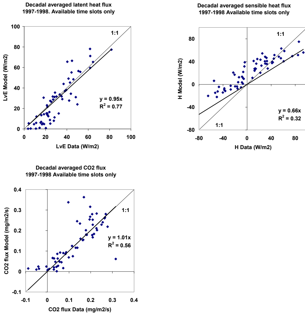
Figure 3.10: Scatter plots comparing model output with measurements for Loobos with A_{m,max}(@25)=1.0 \text{ mg/m}^2/\text{s} , g_m(@25)=3.2 \text{ mm/s} , f_0=0.90 and a_d=-0.12 \text{ kPa}^{-1} .
