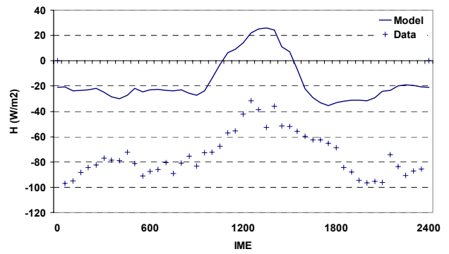
Diurnal cycle of sensible heat flux 199802
